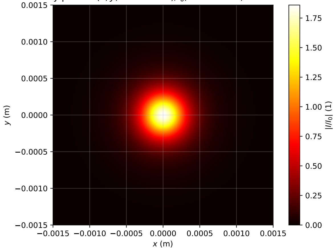
Intensity profile I(x, y, z = 1.513m)/I_0 , P_{in}=1.0P_{cr} , artificial time
